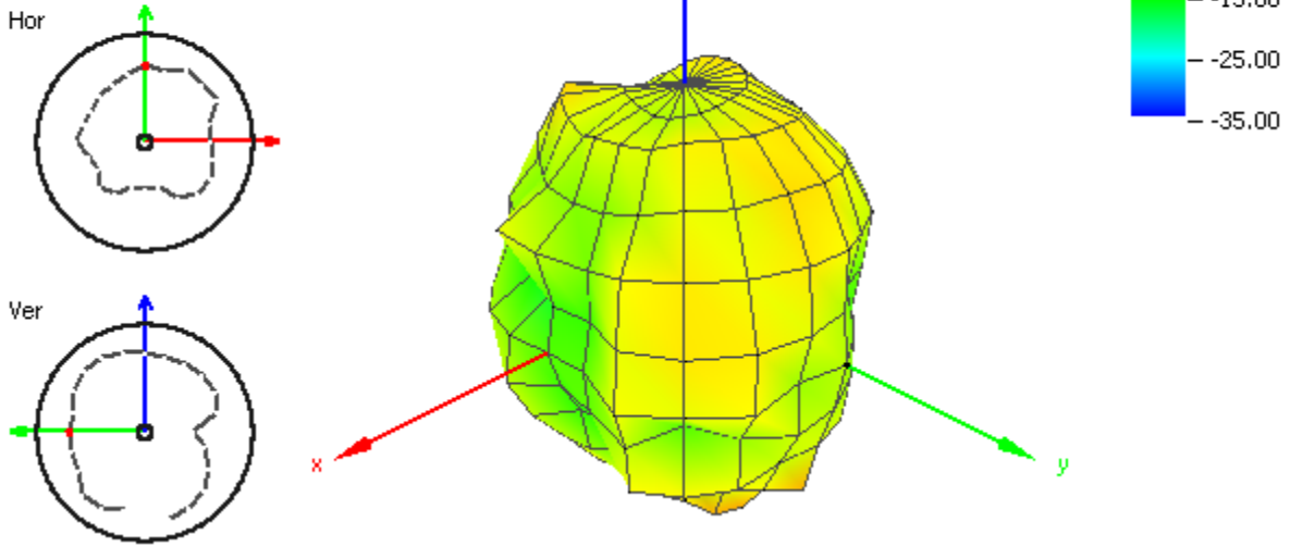
Figure 36. Radiation Pattern at 2400 MHz of G30 Antenna on 30x30cm metal plate.
