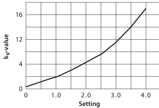
Flow characteristics
