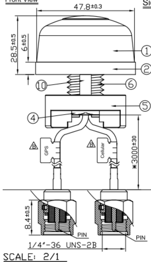
Front View
