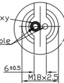
Bottom Thread View
