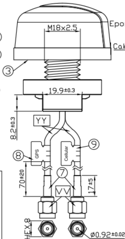
Side View
