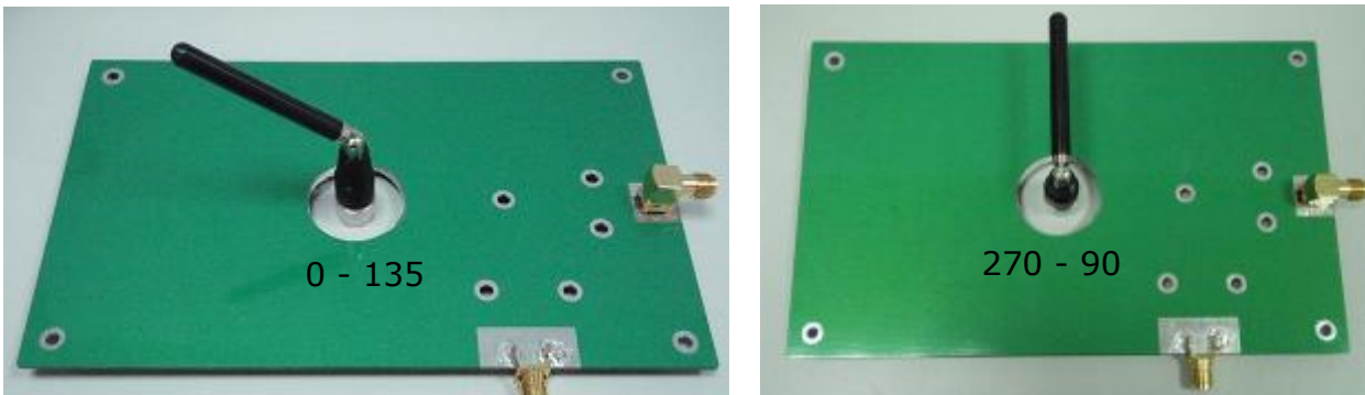
Different antenna mounting is marked as ( \emptyset angle-- \theta angle ), photos are two example of the position marking.
