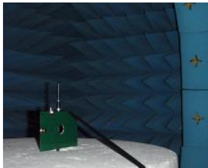
3. Mounting Upright
