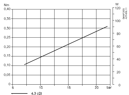
Operating torque
