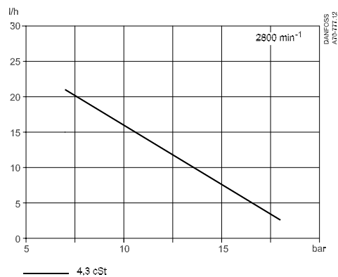
Nozzle capacity
