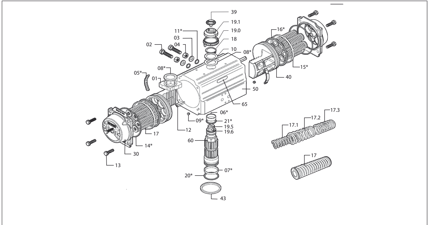
Fig. 6: Component overview
