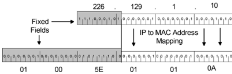
Mapping of class D 226.129.1.10 IP address to MAC layer multicast
